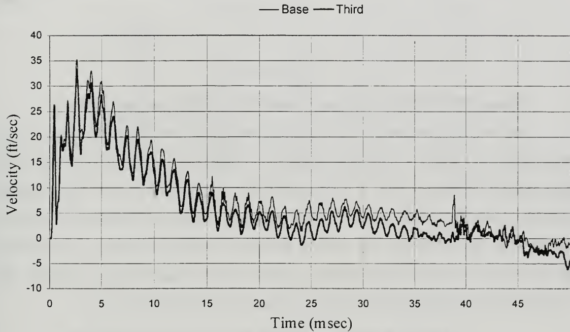
Figure 28: Vertical Response of Node 159 for Base and Half Models
