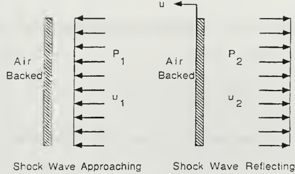
Figure 3. Taylor Plate Subjected to a Plane Wave [Ref. 9]
