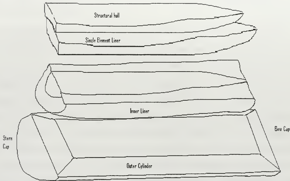
Figure D1: Sketch of Modeling Scheme
