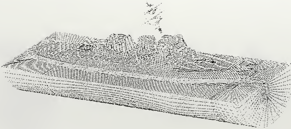
Figure D9: Coupled Ship and Fluid
