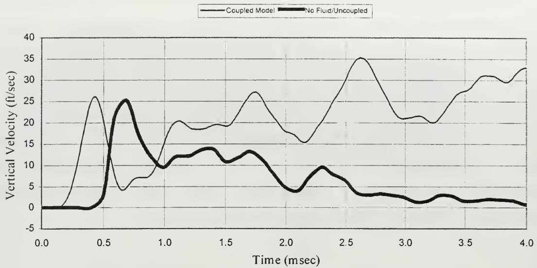
Figure E2: Initial 4-msec of Response of Node 159
