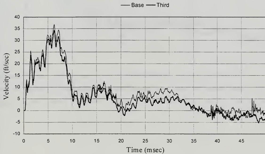
Figure 27: Vertical Response of Node 25 for Base and Half Models
