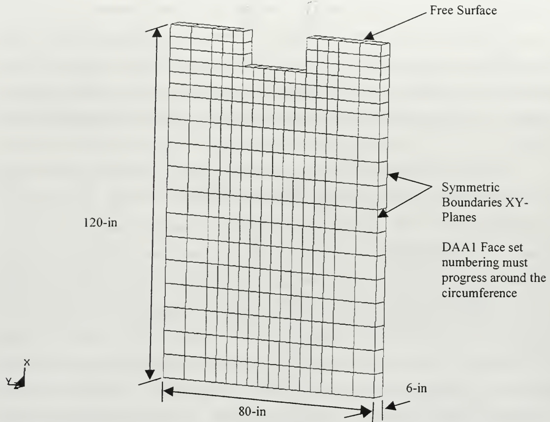
Figure 7: 2-D Fluid Model with Barge Cross-section
