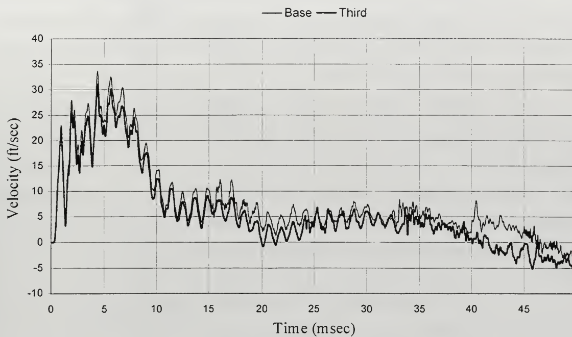
Figure 31: Vertical Response of node 398 for Base and Half Models
