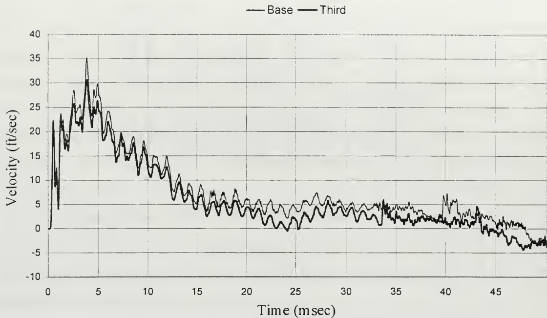
Figure 29: Vertical Response of node 285 for Base and Half Models
