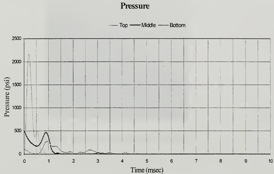
Figure 17: 2D Pressure Response
