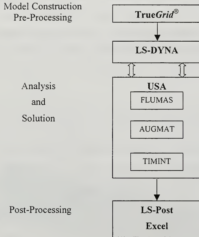
Figure 9: Flow Chart. Model Construction and Simulation
