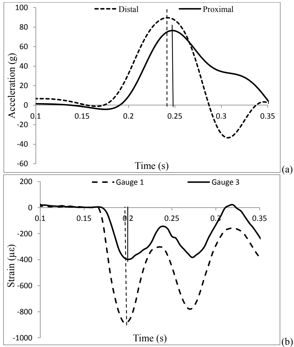
Figure 2.10: Acceleration and Strain Curves
