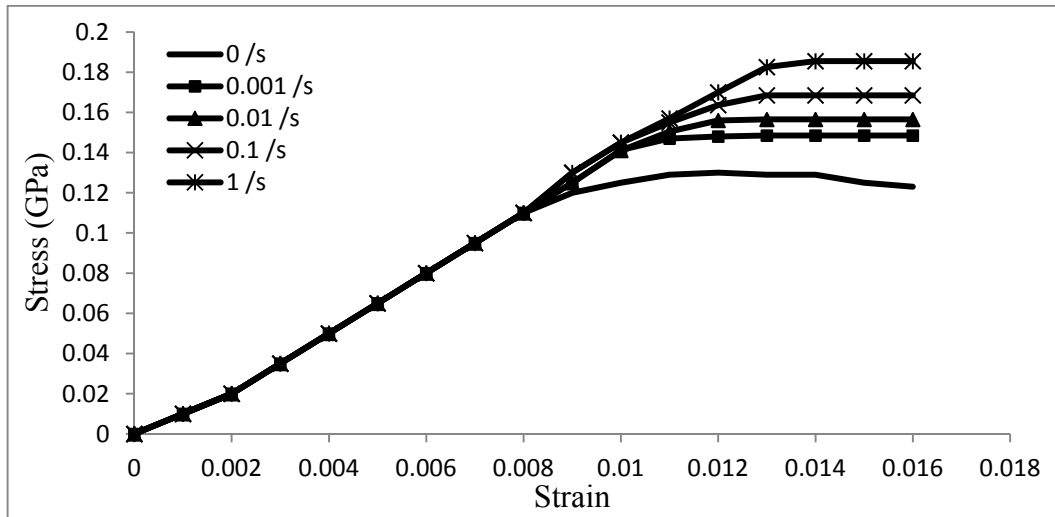
Figure 4.13: Cowper-Symonds Strain Rate Effects
