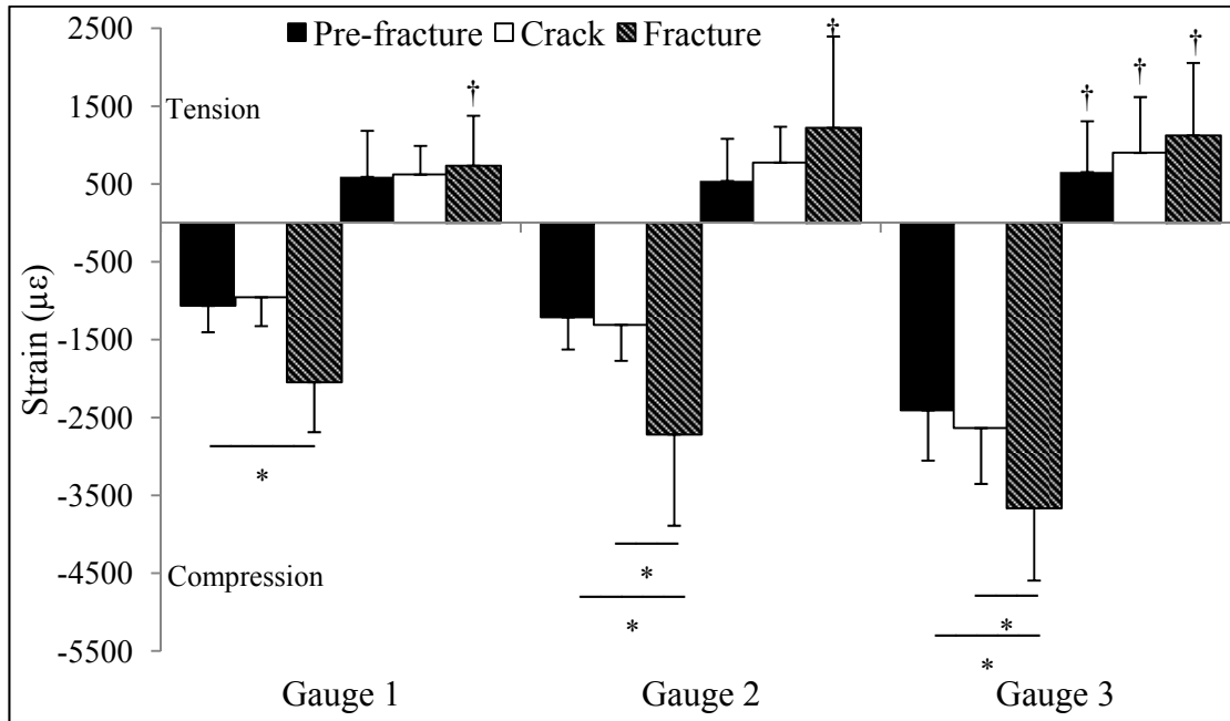
Figure 2.4: Radius Strains
