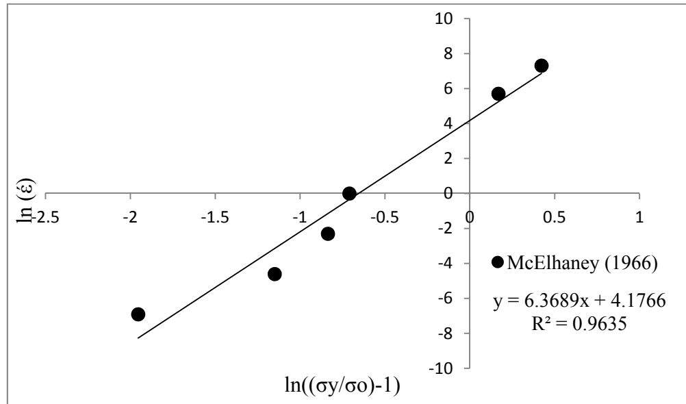
Figure 4.15: Cowper-Symonds Parameters
