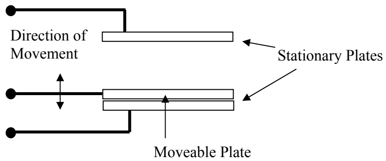
Figure 1.11: Accelerometer Structure
