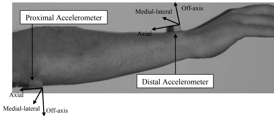
Figure 3.5: Experimental Accelerometer Placement
