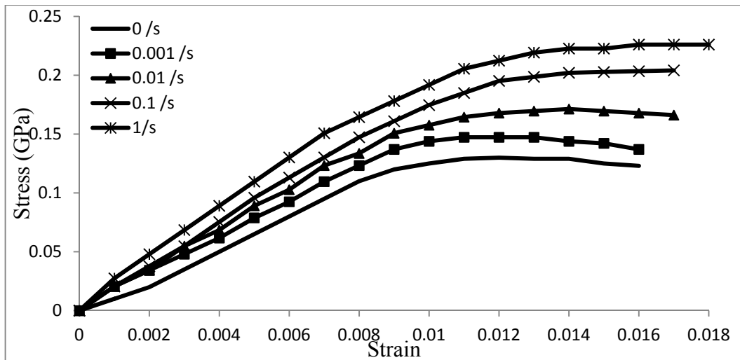
Figure 4.14: Family of Curves Strain Rate Effects
