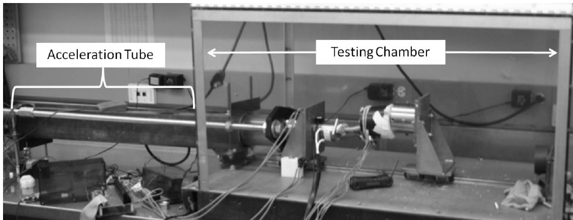
Figure 2.2: Impactor Set-up
