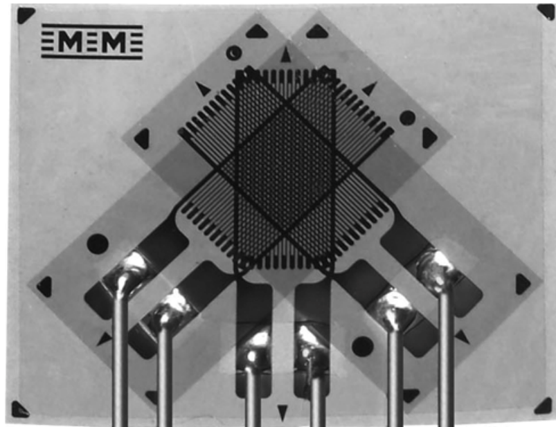
Figure 1.10: Strain Gauge Rosette
