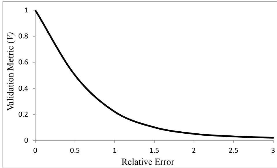
Figure 4.17: Validation Metric
