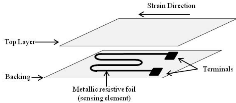
Figure 1.9: Strain Gauge Structure
